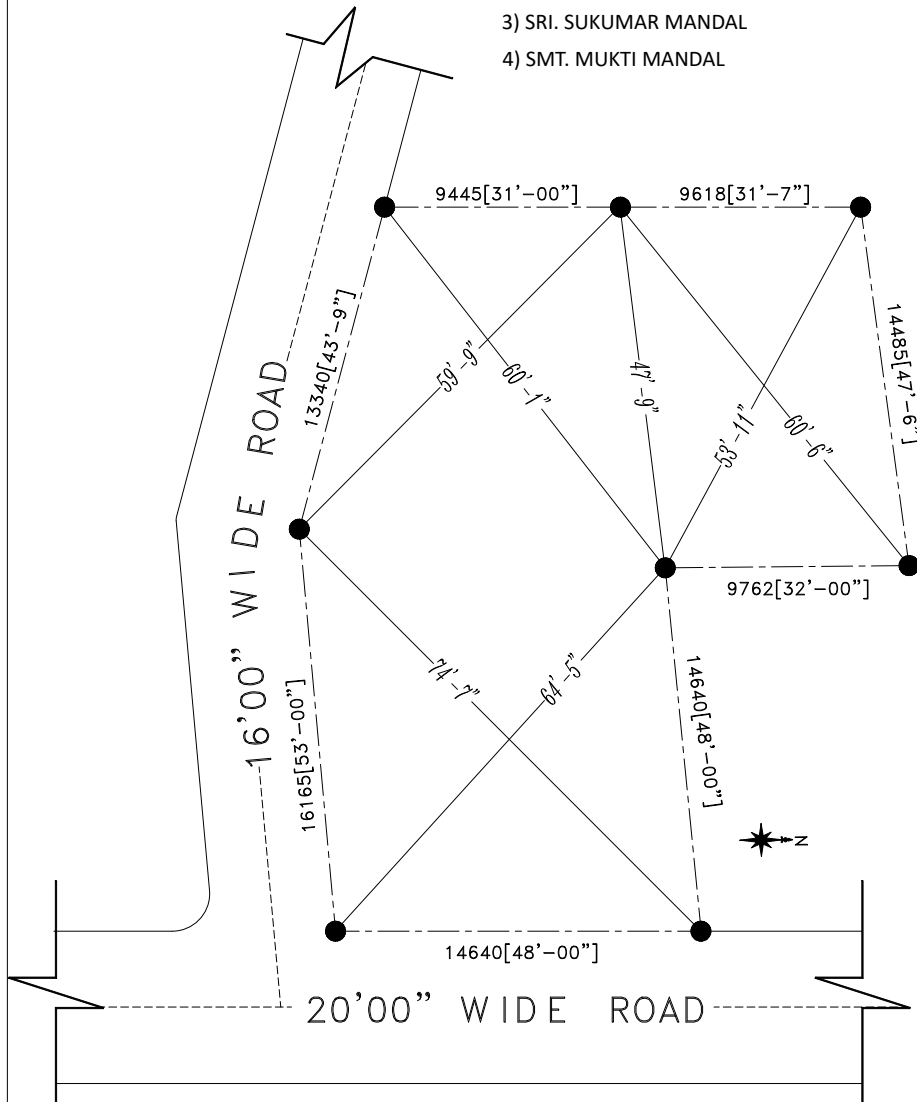
LAYOUT MAP 1:100
